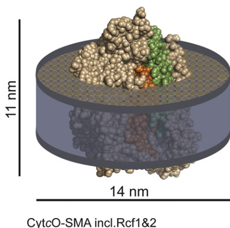
Fig. 7. Schematic model of a CytcO-lipid SMA native nanodisc. The CytcO structure is based on a model of yeast CytcO [28] and prepared using the software PyMol [59]. Subunits I and II are shown in orange and green, respectively. The picture illustrates the approximate proportions of the lipid disc and of the protein.
