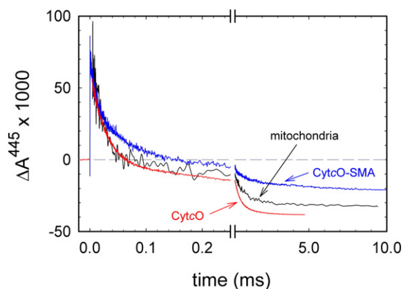
Fig. 5. Absorbance changes associated with reaction of reduced Cyt c O with O 2 . The reaction was studied with three samples: Cyt c O in SMA native nanodiscs (blue), in native membranes (grey) and in the detergent DDM (red). The O 2 concentrations after mixing were 0.9 mM, 0.6 mM and 0.6 mM, respectively. For experimental conditions, see Fig. 4. The CO ligand was dissociated by a laser flash at a time ~200 ms after mixing (the flash defines t = 0 ). All amplitudes were normalized to 1 μM reactive enzyme. The rate constants were determined using the software ProK.
