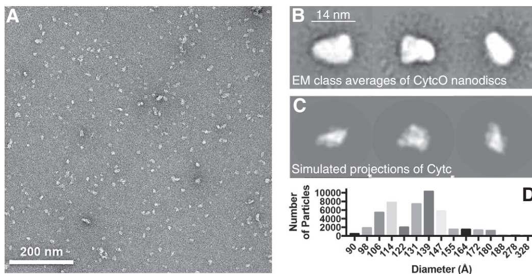
Fig. 1. Negative stain EM of CytcO-SMA native nanodiscs. (A) Representative negative stain EM image of CytcO-SMA native nanodiscs showing regularly sized and monodisperse complexes. (B) Representative 2D class averages of CytcO-SMA native nanodisc particles. Each class average contains \sim 100 particles. (C) Projections of crystal structure of bovine CytcO in three different views, scaled to the same pixel size as in panel (B). (D) Distribution of particle sizes obtained for 46,764 CytcO-SMA native nanodiscs particles.
