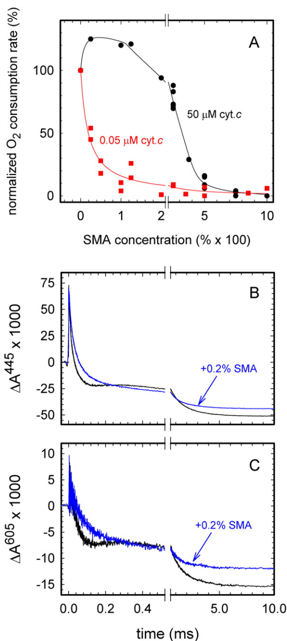
Fig. 6. Effect of SMA on the activity of CytcO. (A) Steady-state O 2 -reduction activity of the S. cerevisiae mitochondria in the presence of SMA. The activity is defined by the oxygen-consumption rate measured with equine heart cyt. c at 50 μM (black dots) or 0.05 μM (red squares). The activity is presented as relative values compared to that in the absence of SMA (set as 100%). The 100% activities were 250 e - /s and 70 e - /s, respectively. The IC 50 values for 50 μM and 0.05 μM cyt. c were 0.032 10 -2 % and 0.0019 10 -2 %, respectively. The concentration of yeast mitochondria protein was 0.2 mg/ml. For other experimental conditions, see the Materials and Methods section. (B,C) Reaction of fully reduced bovine CytcO with oxygen in the absence (black traces) and in the presence (blue traces) of 0.2% SMA, monitored at 445 nm (B) and 605 nm (C). The O 2 concentration after mixing was 0.9 mM. The buffer contained 0.1 M KCl, 20 mM HEPES (pH 8.0), 0.1 mM EDTA and 0.05% DDM. For other experimental conditions, see Fig. 4. The CO ligand was dissociated by a laser flash at t = 0, ~200 ms after mixing. All amplitudes were normalized to 1 μM reactive enzyme. The rate constants were determined using the software ProK.
